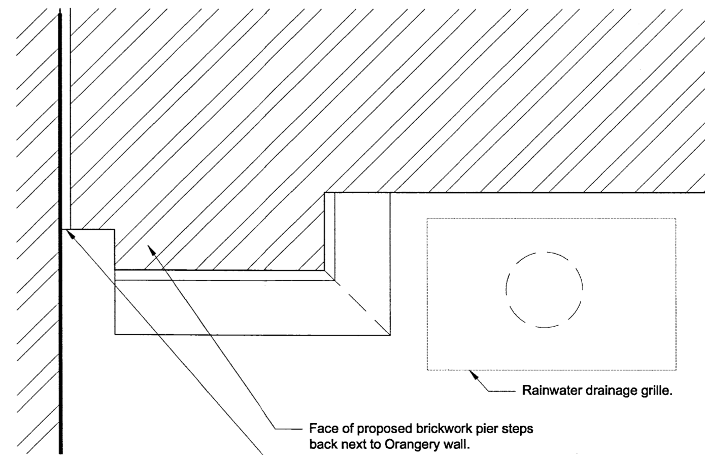
DETAIL B. PLAN_(1:5)
