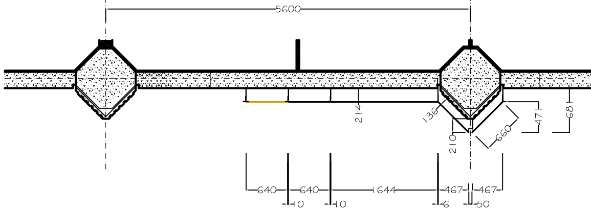
Enlarged Plan View. Scale- 1:20
