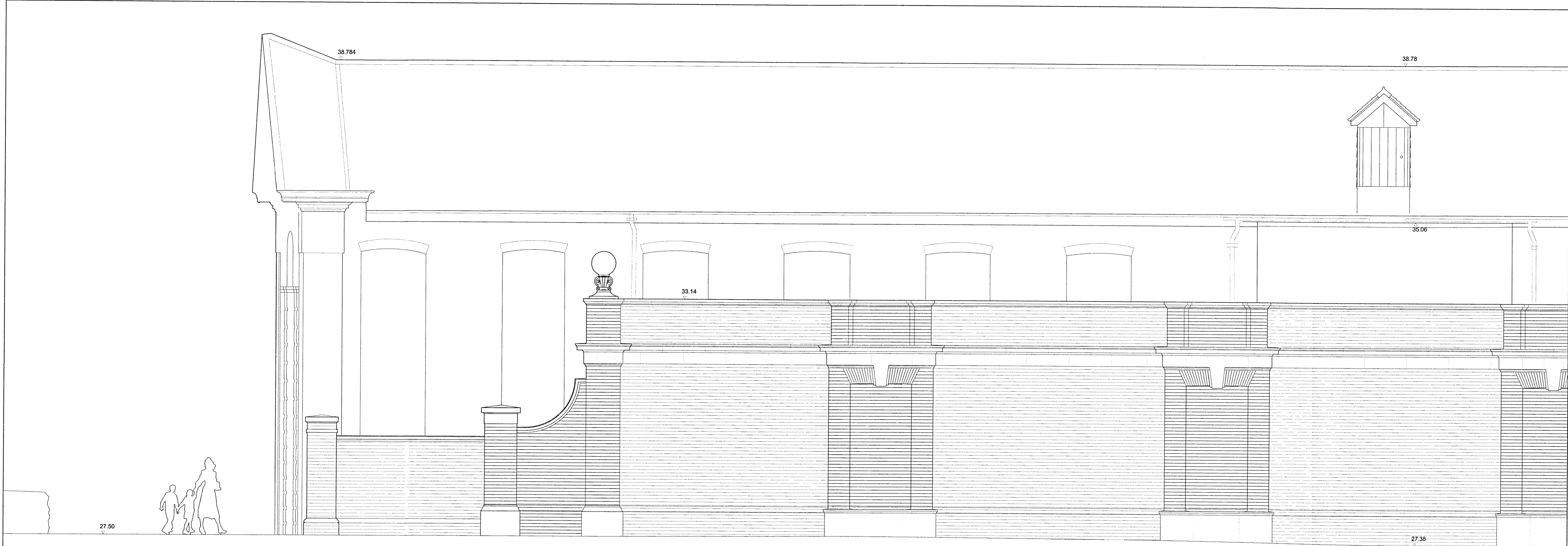
PROPOSED BUILDING PARTIAL ELEVATION_1-50 (@A1)
