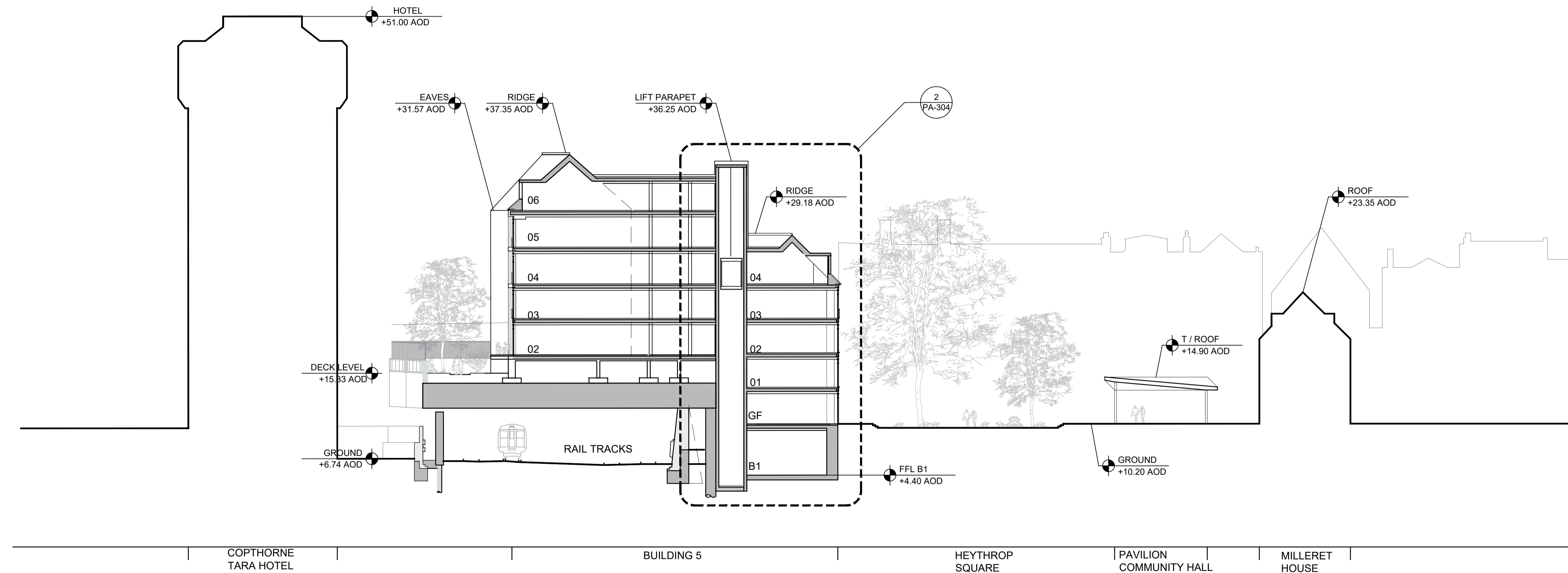
2 EAST-WEST SECTION 2 SCALE: 1:250
