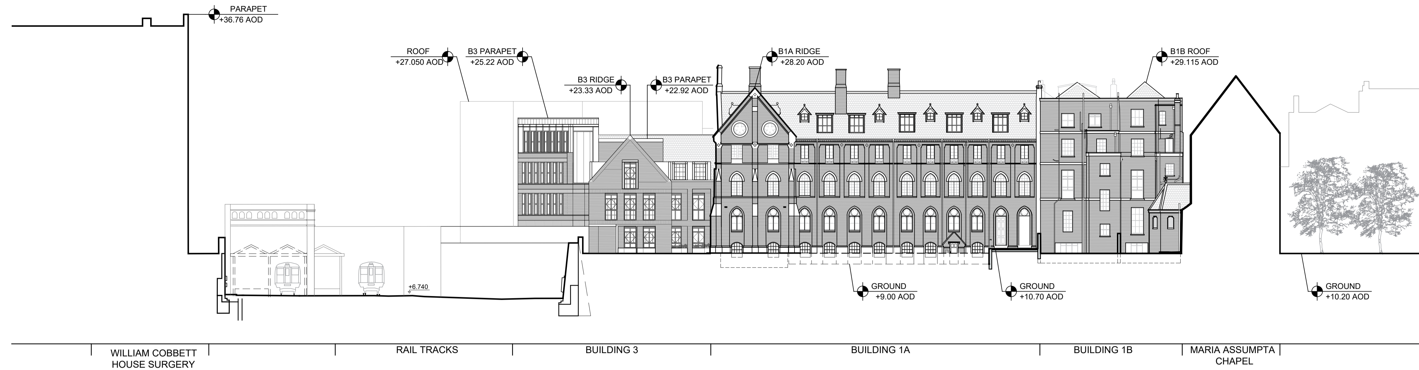
1 EAST-WEST SECTION 1 SCALE: 1:250
