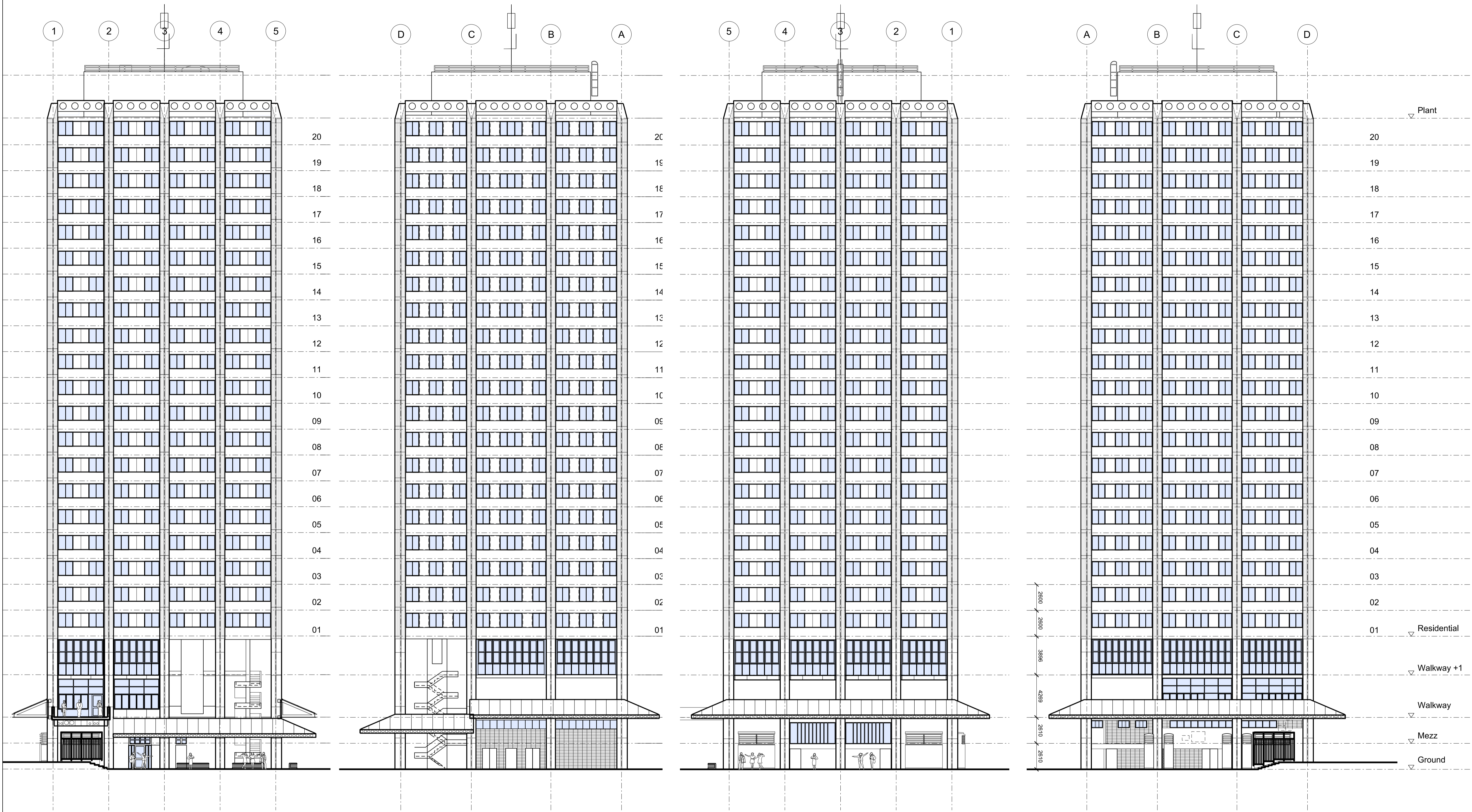
1 SOUTH ELEVATION 1:200
