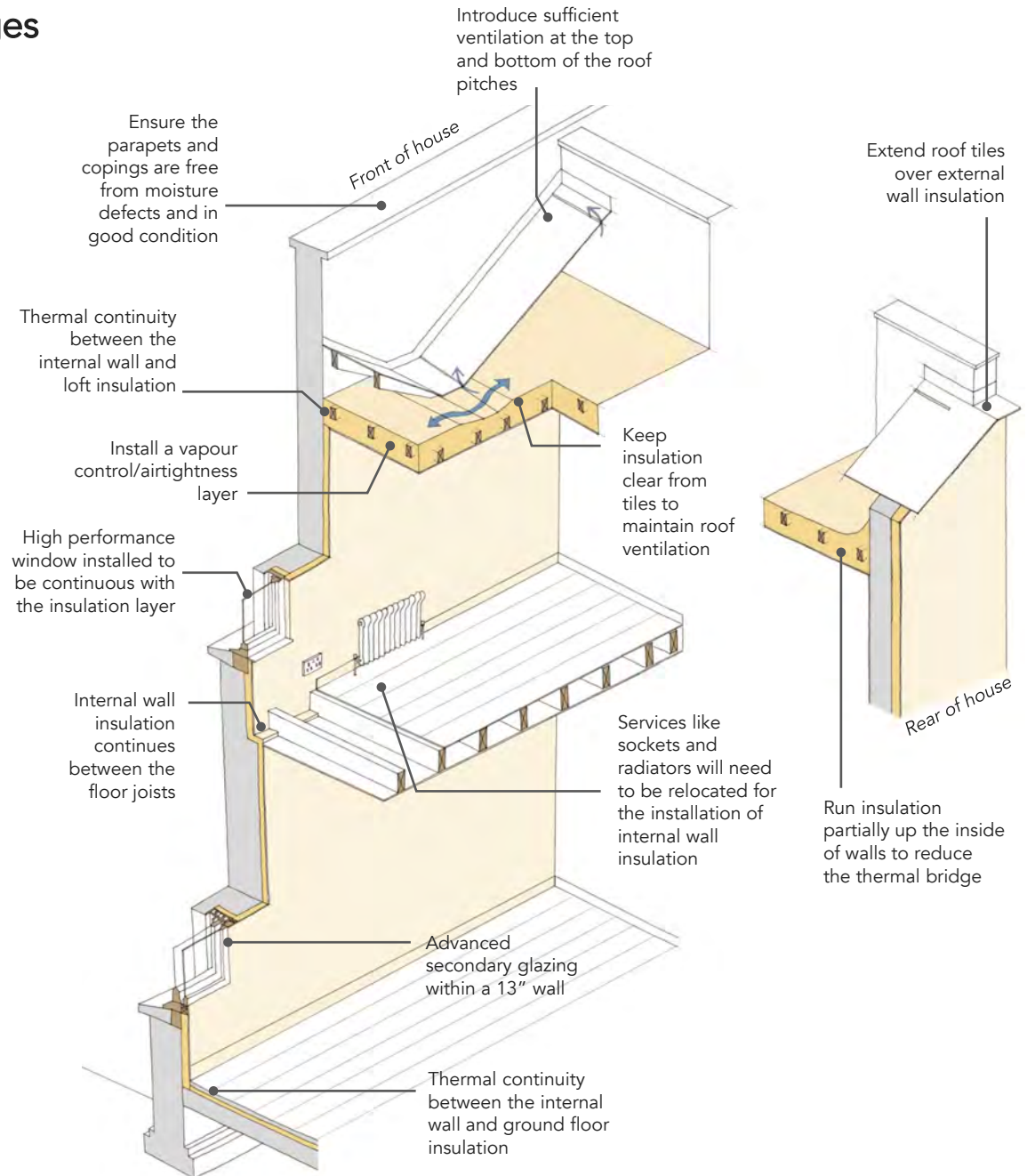
Butterfly roof to wall to ground junctions – front and rear of home
