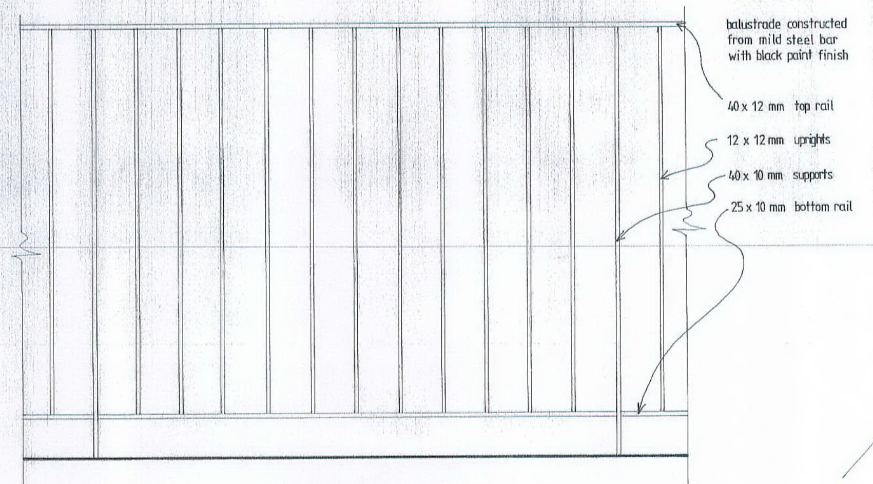
elevation of proposed new balustrade 1:10
