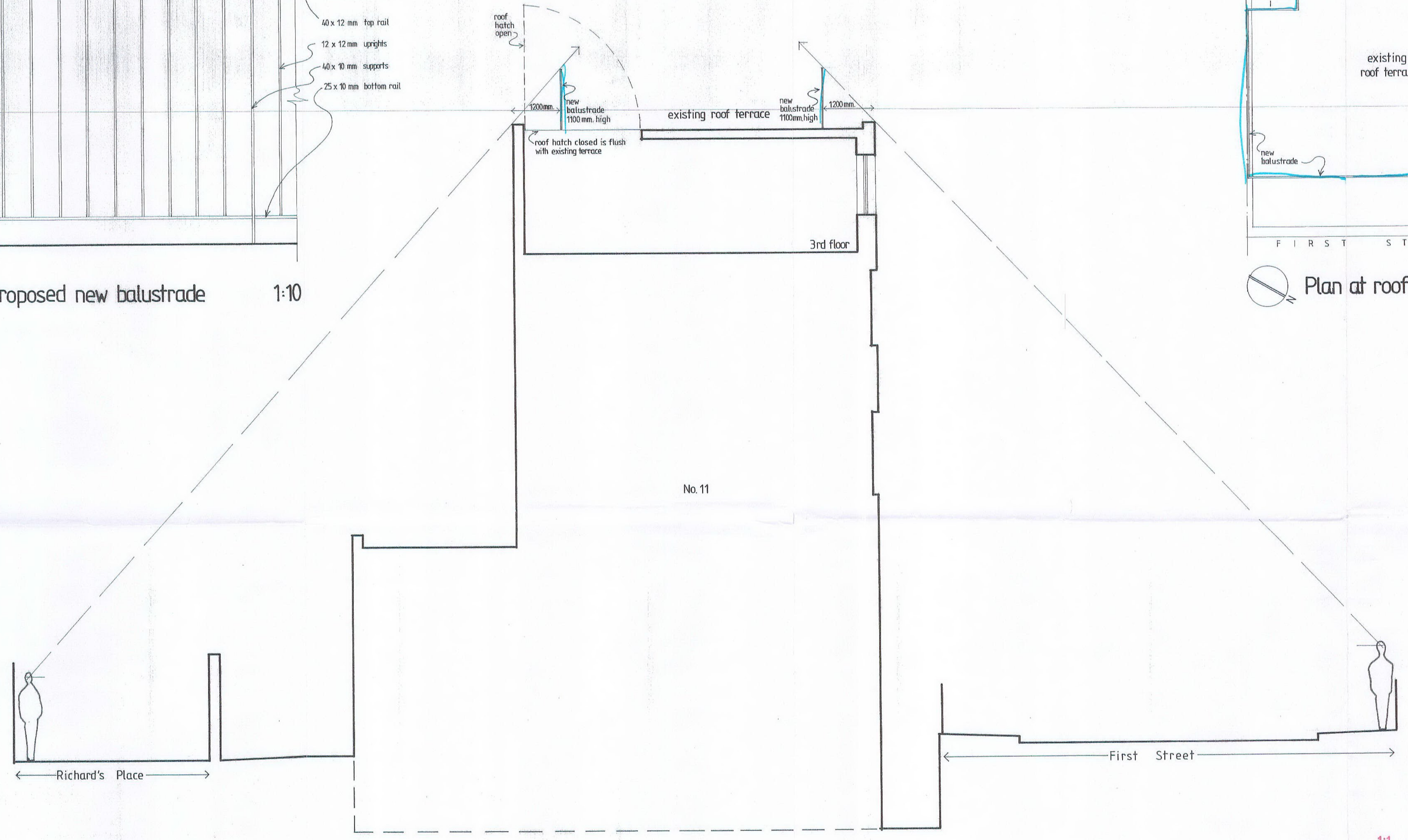
Diagram cross section
