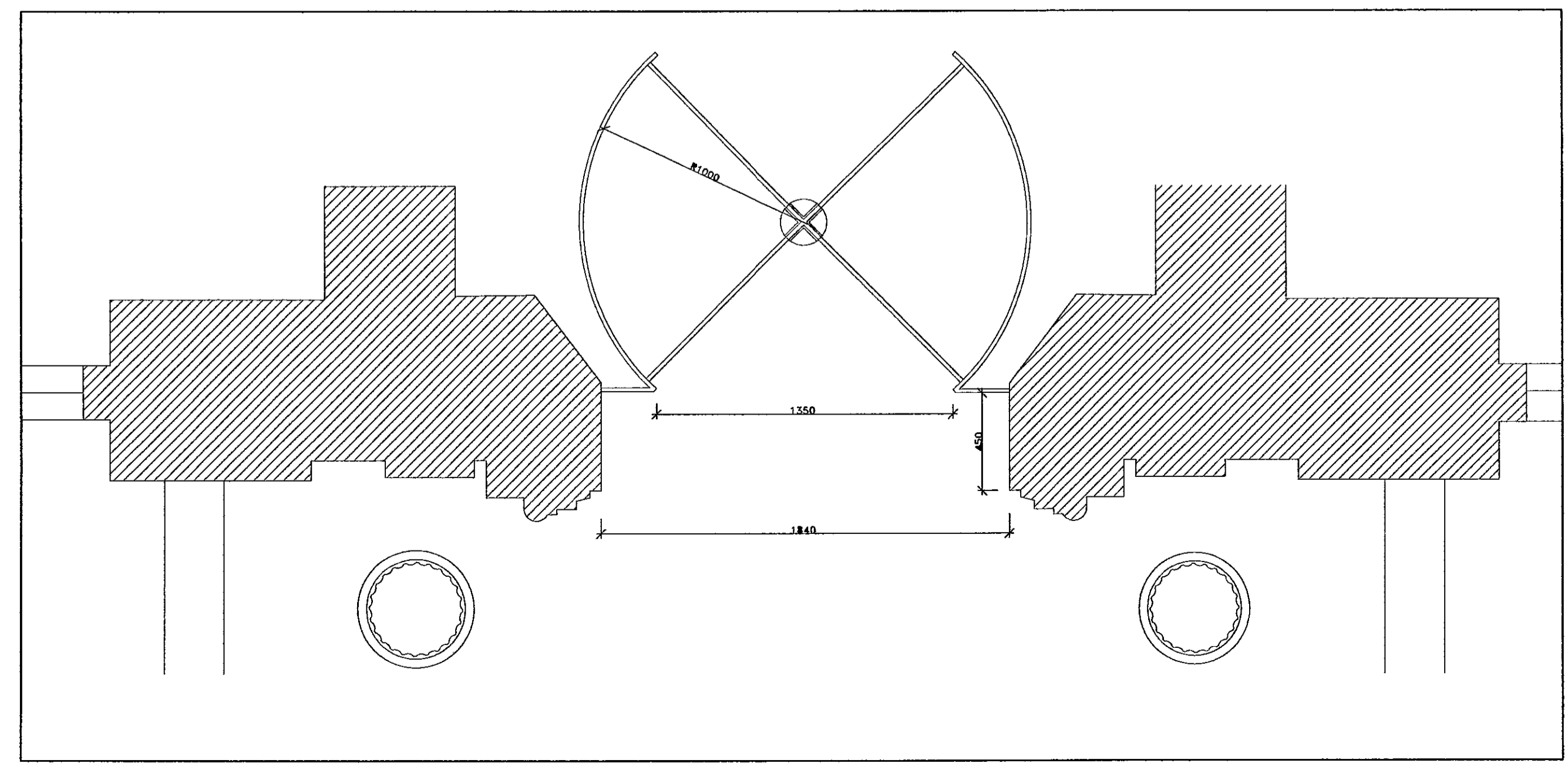
PROPOSED REVOLVING DOOR PLAN
