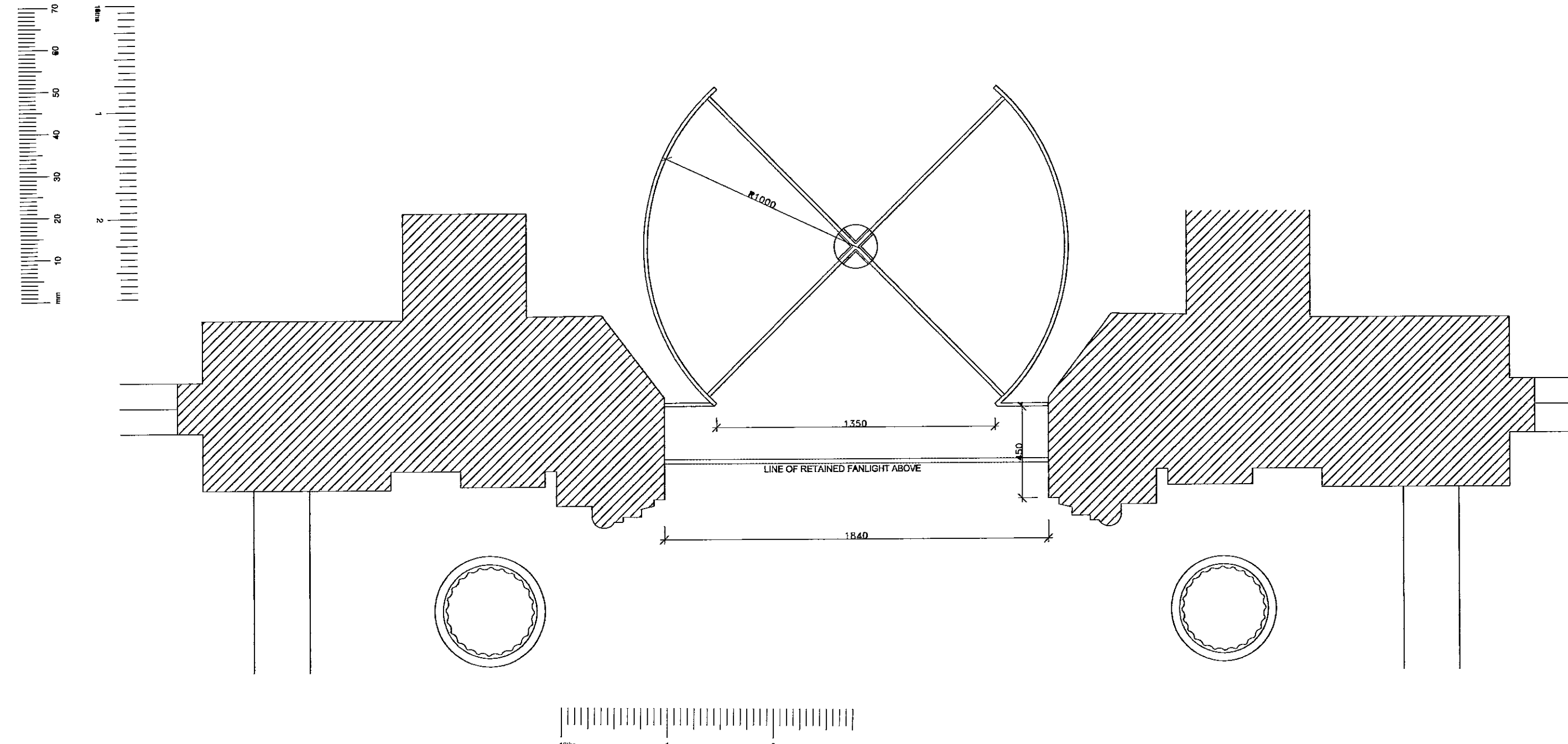
PROPOSED REVOLVING DOOR PLAN
