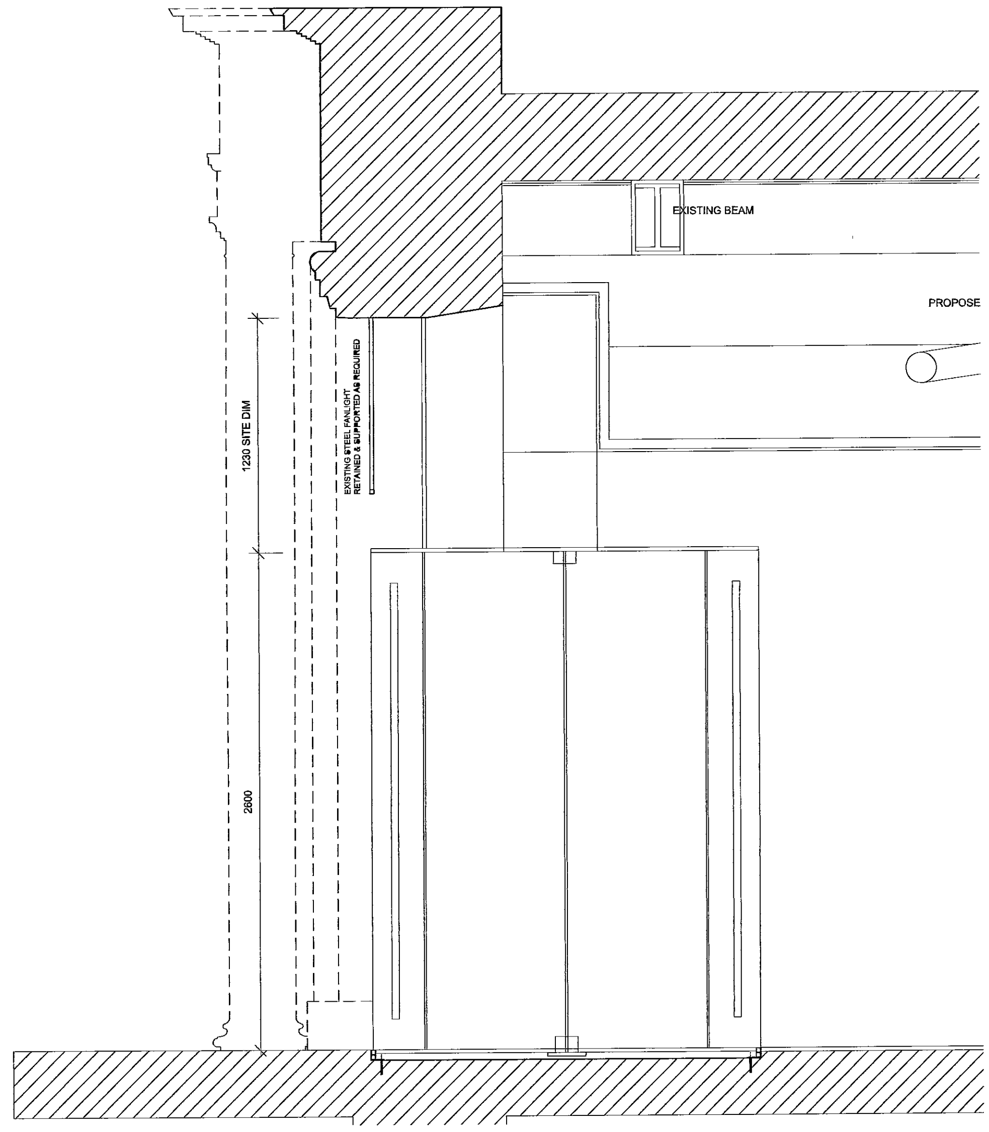
PROPOSED REVOLVING DOOR SECTION
