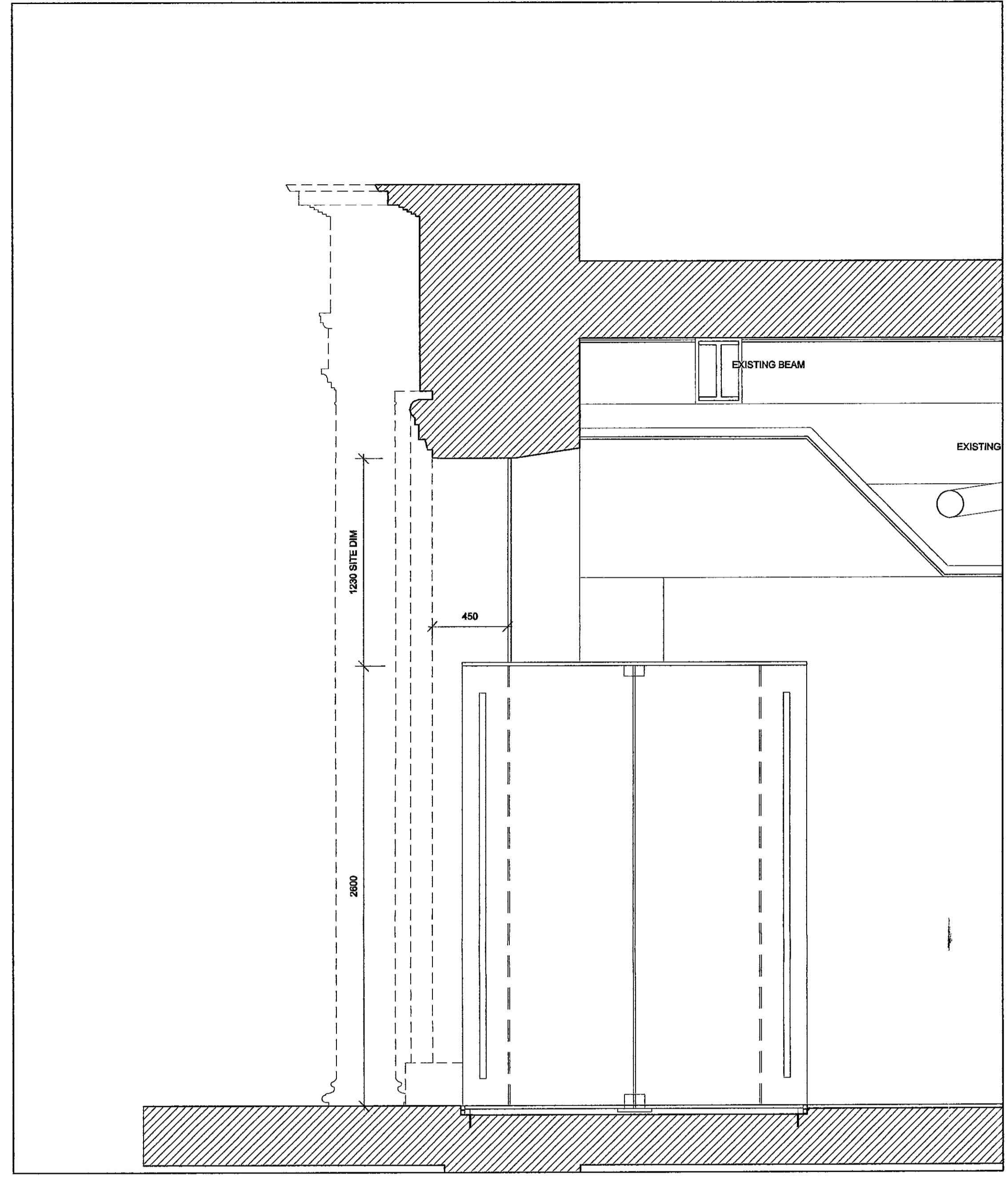
PROPOSED REVOLVING DOOR SECTION
