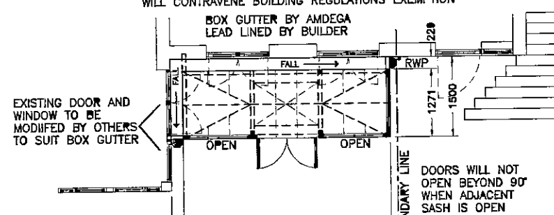
PROPOSED PLAN VIEW
