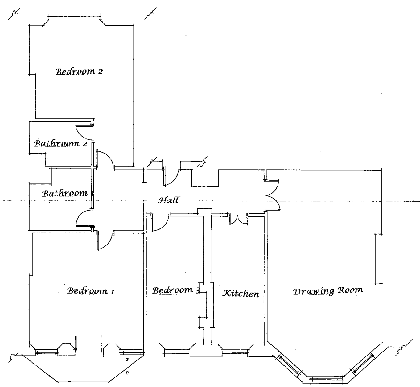
Existing Layout
