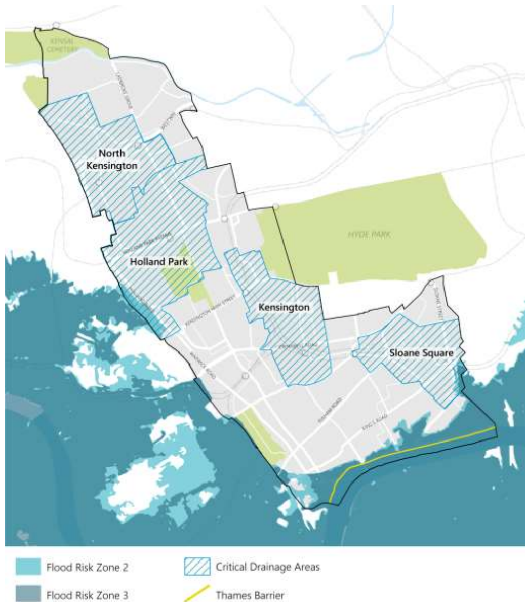
Figure 2.22.2: Flood Risk Zones, Critical Drainage Areas and Thames Barrier
