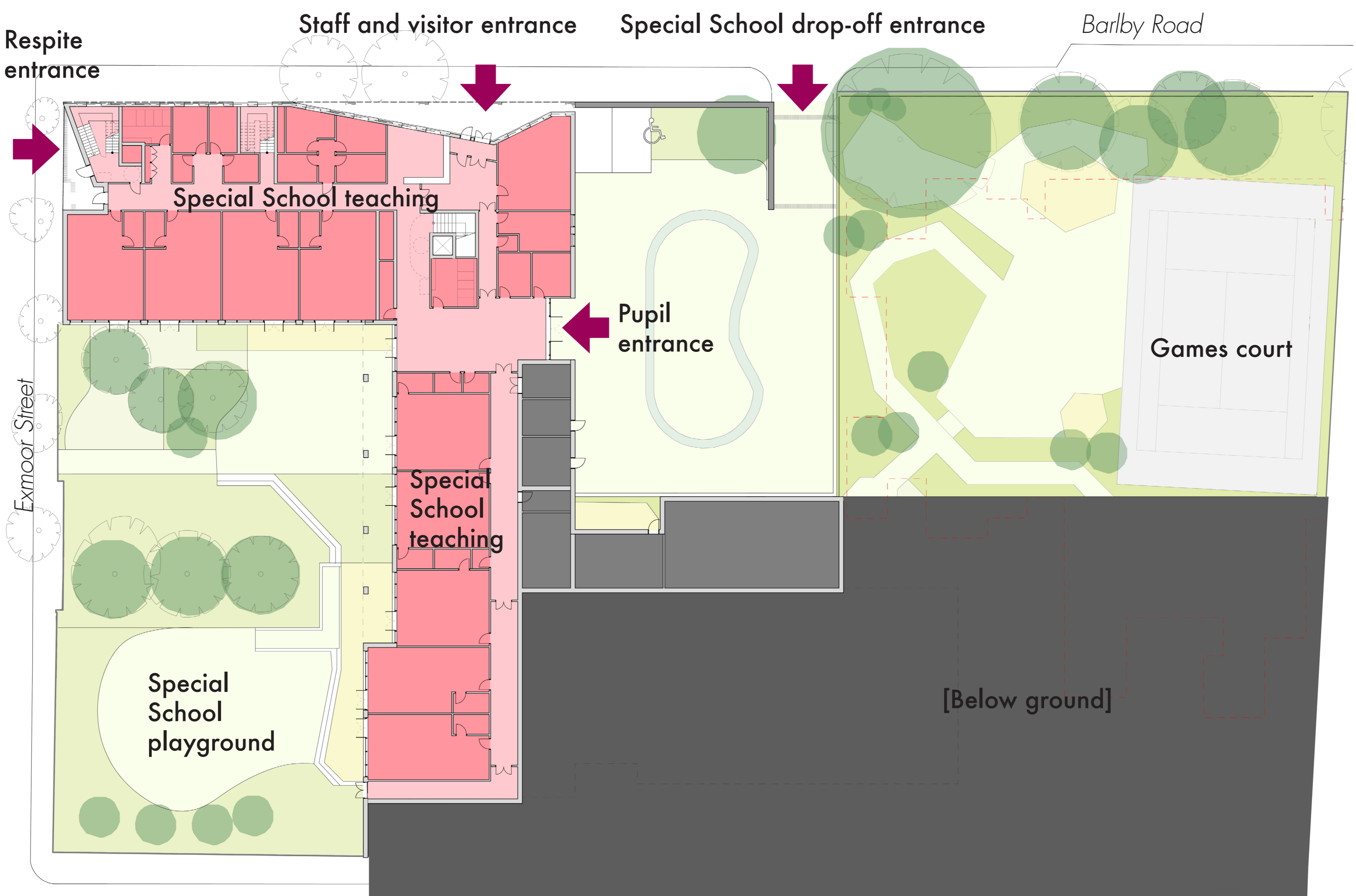
Lower ground floor plan - Exmoor Street level
