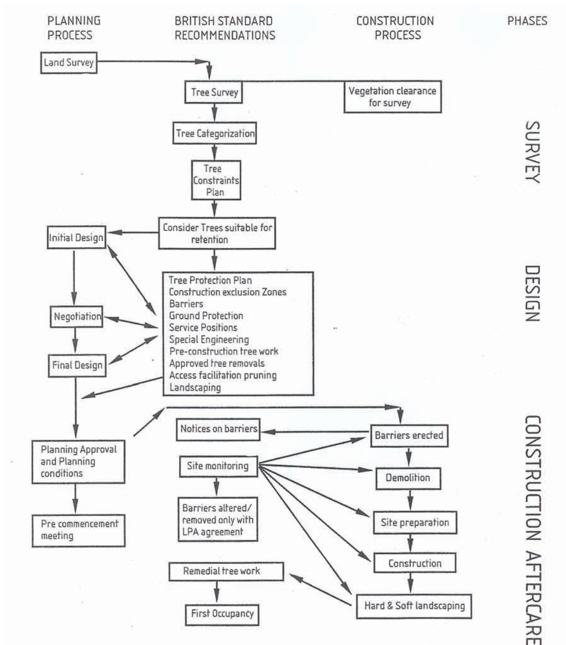
Figure 1. Flow diagram, summarizing planning for trees on development sites (extract from BS 5837: 2005)
